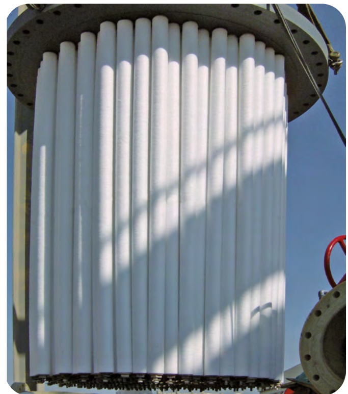
Removal of filter pack in a desalination plant in Algeria. Production capacity: 200,000 \text{m}^3/\text{d} .
